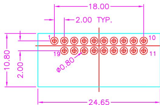
P.C.B LAYOUT TOP VIEW ±0.05
