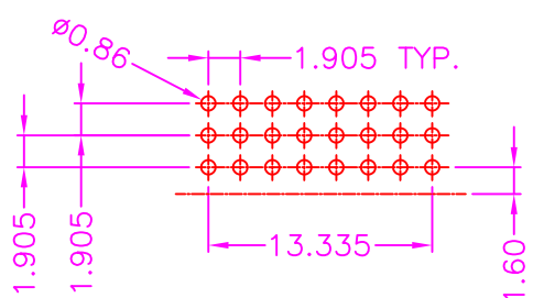
P.C.B LAYOUT TOP VIEW ±0.05
