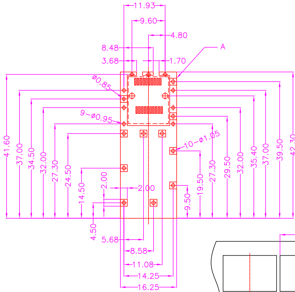
P.C.B LAYOUT TOP VIEW ±0.05
