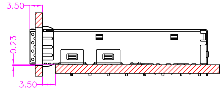
BEZEL OPENING BELOW TOP OF PCB
