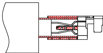
MATED CONDITION
