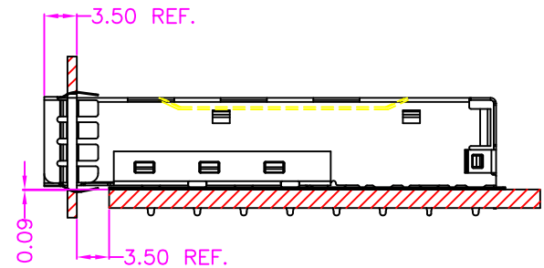
BEZEL OPENING BELOW TOP OF PCB
