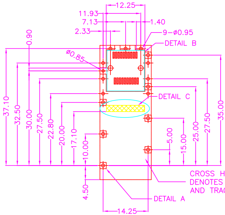
P.C.B LAYOUT TOP VIEW ±0.05
