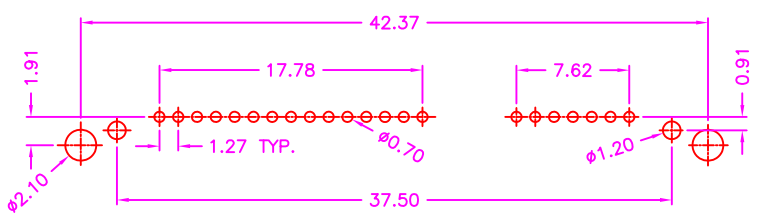
P.C.B. LAYOUT TOP VIEW ±0.05
