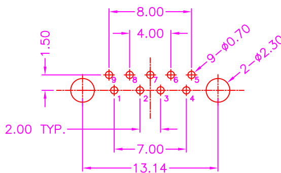
P.C.B. LAYOUT TOP VIEW ±0.05
