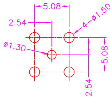
P.C.B. LAYOUT TOP VIEW ±0.05
