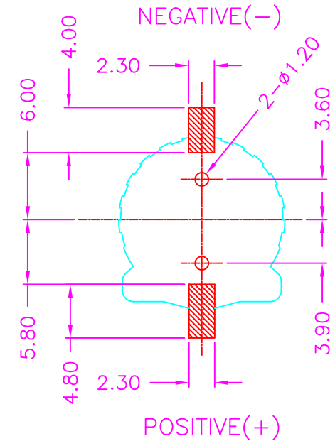
P.C.B LAYOUT TOP VIEW ±0.05
