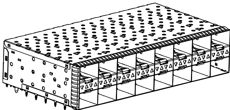
F28BK-0*C-111 WITH INNER & OUTER LIGHT PIPES
