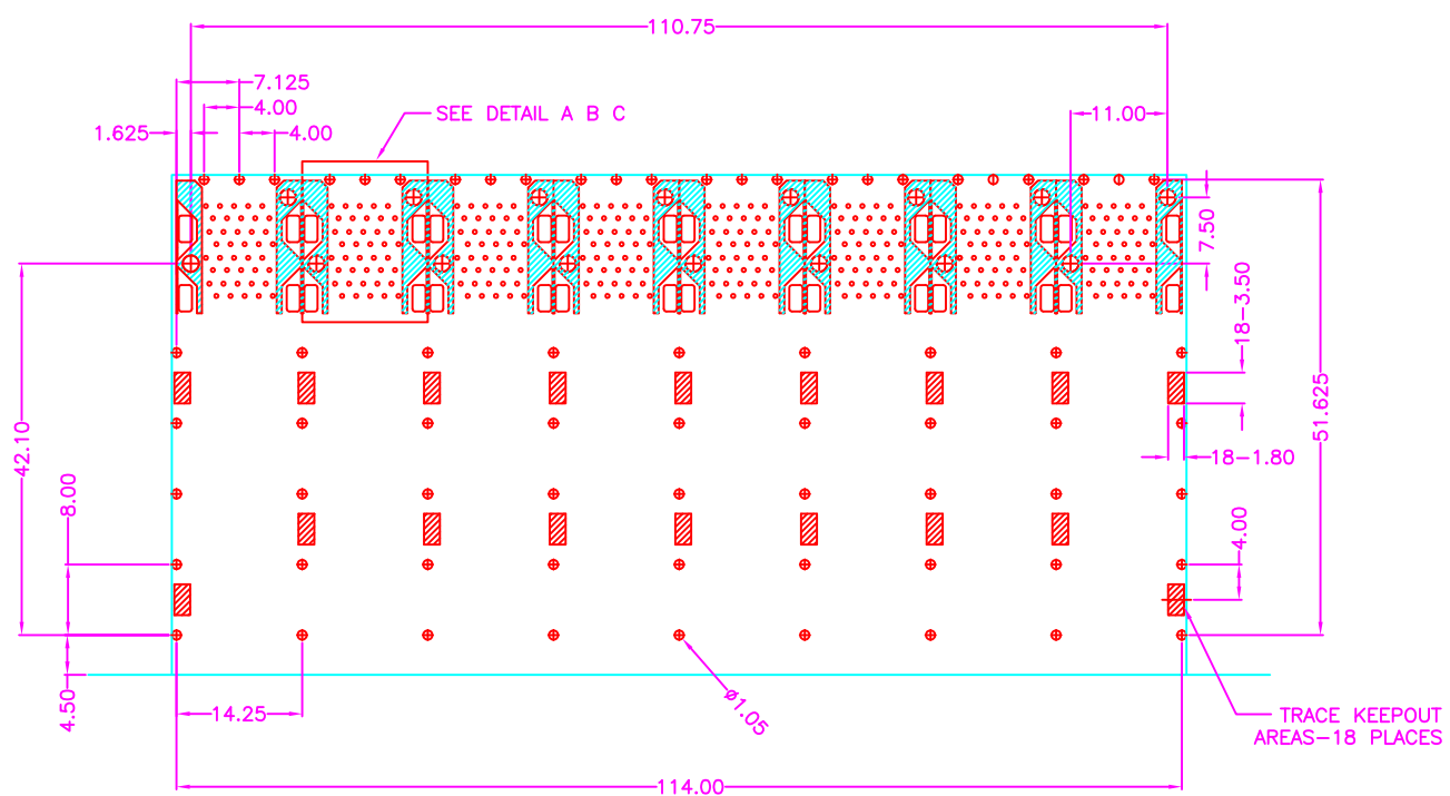
P.C.B LAYOUT TOP VIEW ±0.05
