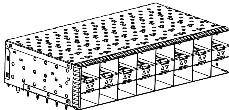
F28BK-0*C-131 WITH INNER LIGHT PIPES
