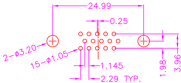
P.C.B LAYOUT TOP VIEW ±0.05
