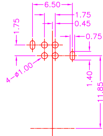
P.C.B. LAYOUT TOP VIEW ±0.05
