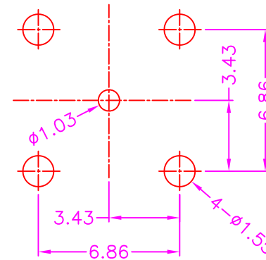
P.C.B. LAYOUT TOP VIEW ±0.05
