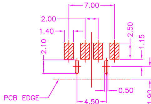
P.C.B. LAYOUT TOP VIEW ±0.05
