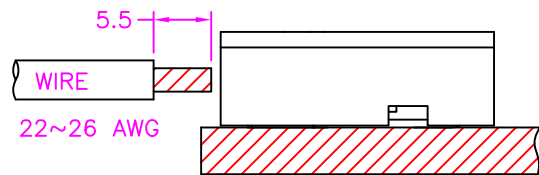
ASSEMBLY
