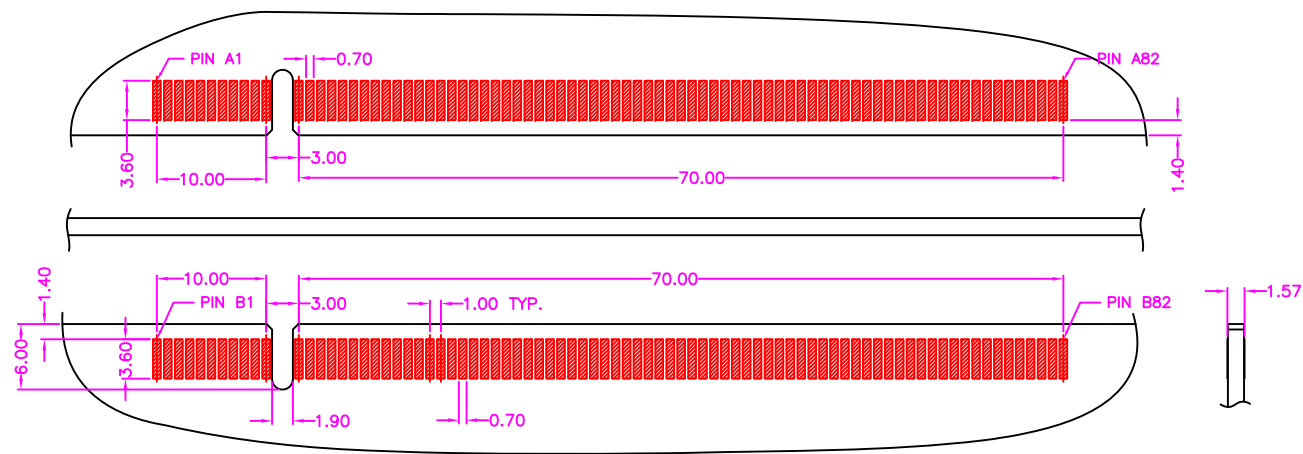
RECOMMENDED OF PCB DIMENSIONS TOLERANCE: \pm 0.05
