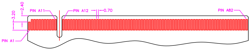
ADD-IN CARD EDGE-FINGER DIMENSIONS TOLERANCE: \pm 0.05
