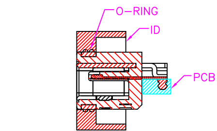
RECESSED MOUNTING CONFIGURATION
