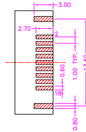
STRADDLE TYPE TOP VIEW P.C.B LAYOUT ±0.05
